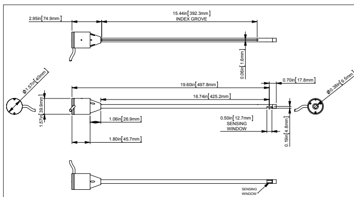
High Intensity UVA Probe
