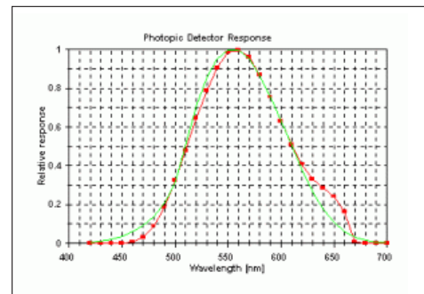
Fig. 1. SL-3101 Photopic Spectral Response
