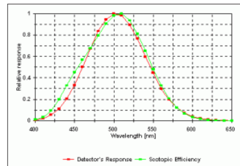
Fig. 2. SL-3101 Scotopic Spectral Response
