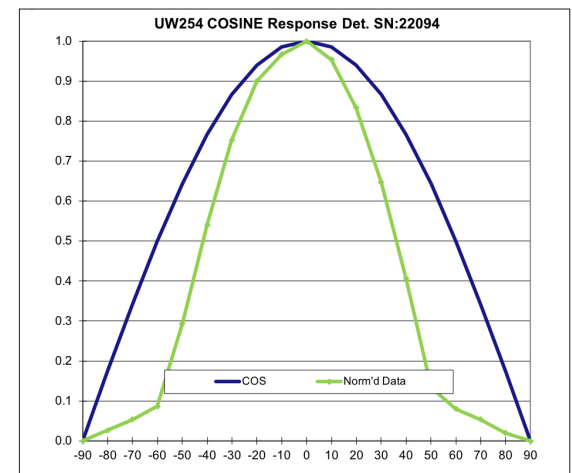
Fig. 3. Cosine Response
