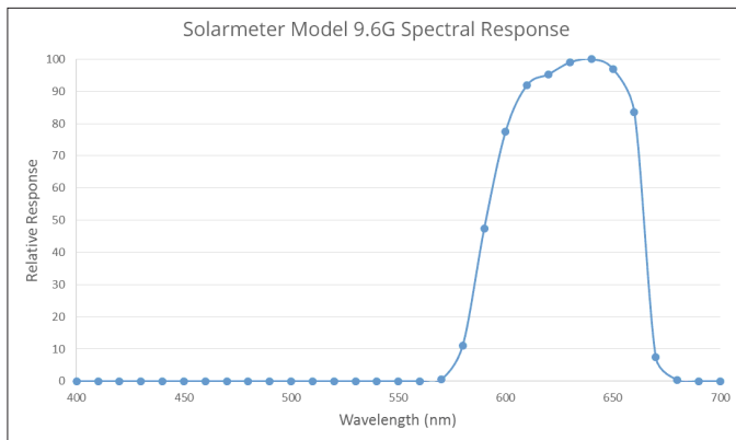
Fig. 1. Model 9.6G Spectral Response
