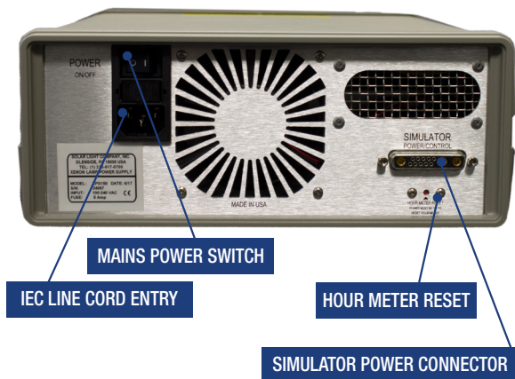
XPS Power Supply Rear Panel
